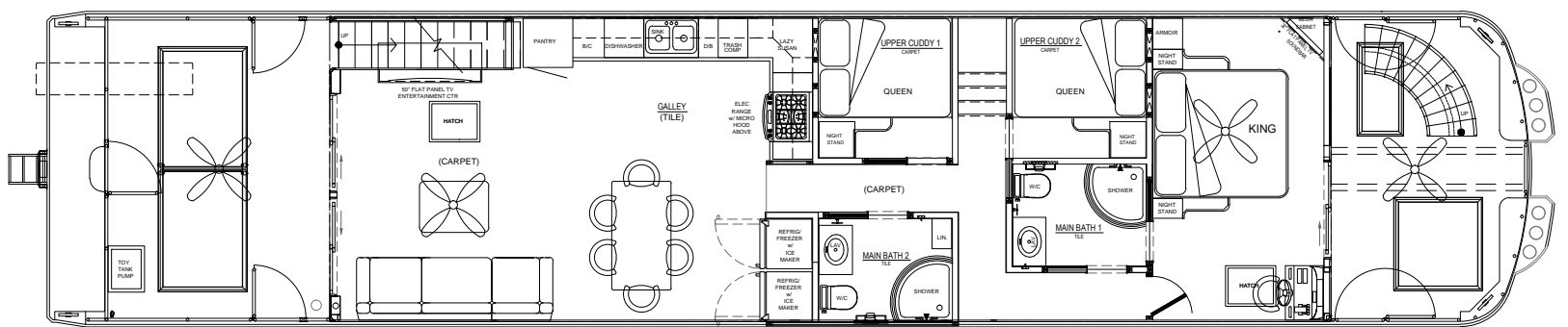
MAIN LEVEL FLOOR PLAN
